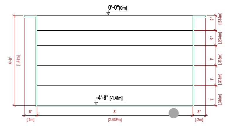
CROSS SECTION B-B
