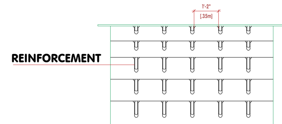
CROSS SIDE VIEW D-D
